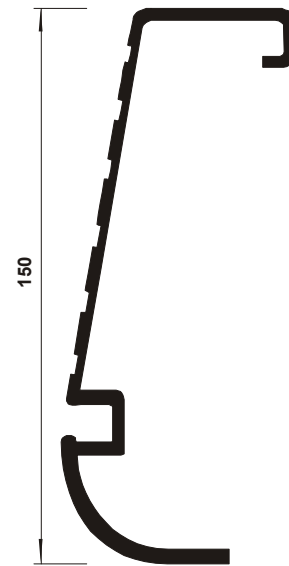
PG 152 Bumpers for Overhaul 150 mm
