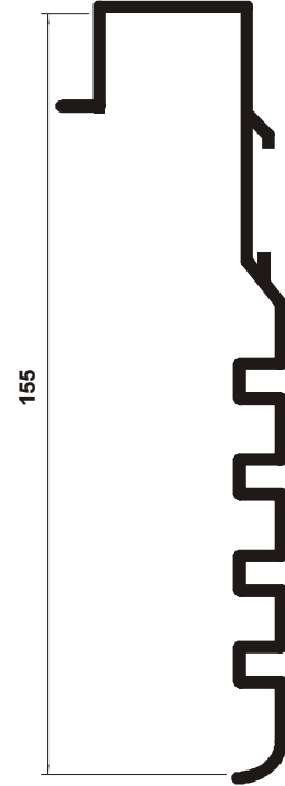
PG 142 Bumpers for Overhaul 155 mm
