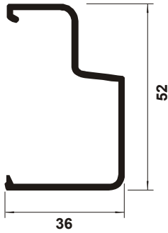
PG 101 Bumpers Stair 52 mm
