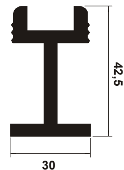
TB 361 Baseboard Double T
