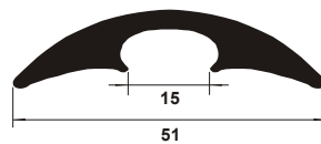
TB 309 Quarterround Joint-cover
