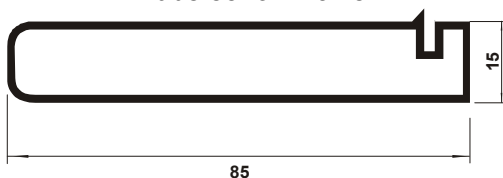
TB 449 Tube 85 for Drawer
