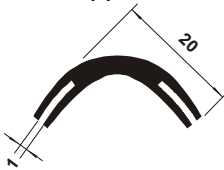
TB 444 Corner Support for 1 mm
