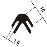
ES 147 Joint Slot - Tongued and Grooved Board
