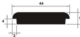
TC 101 Edgebanding 40 Solid
