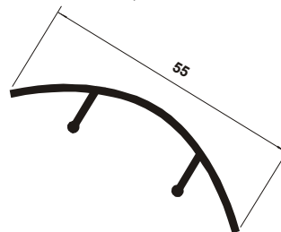
TB 448 Cover Quarterround
