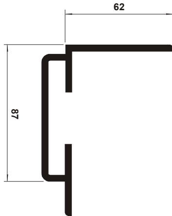
TB 362 Baseboard "L"
