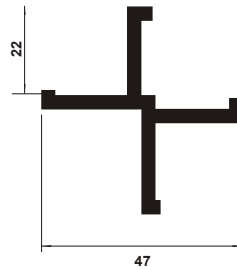
TB 363 Cross 47 sp. 3 mm
