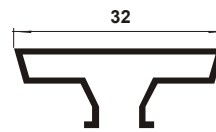
ES 151 Cover Slot Panel
