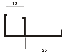
TB 433 Frame Pencil Holder 25 for 13 mm
