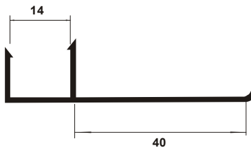
TB 434 Frame Pencil Holder 40 for 14 mm
