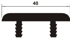
TC 100 Edgebanding 40 with 2 Insertions
