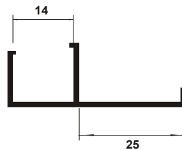
TB 435 Frame Pencil Holder 25 for 14 mm
