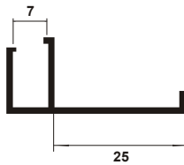
TB 431 Frame Pencil Holder 25 for 7 mm
