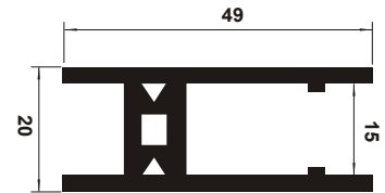
PV 388 Jamb for Leaves
