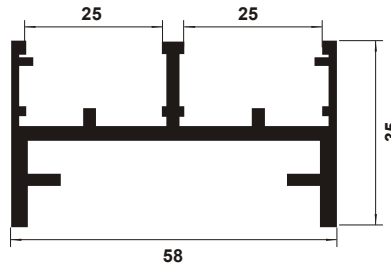
PV 390 Seal to Close Leaves
