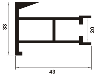
PV 389 Seal to Hook Leaves
