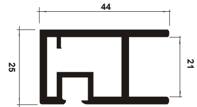
PV 394 Sliding Leaf for Cold
