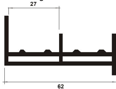
PV 393 Sliding Frame for Cold
