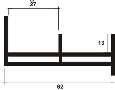
PV 395 Sliding Frame for Cold H 13
