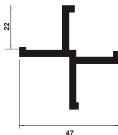
TB 363 Cruz 47 esp. 3 mm
