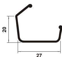
TB 447 Base Quarta Cana
